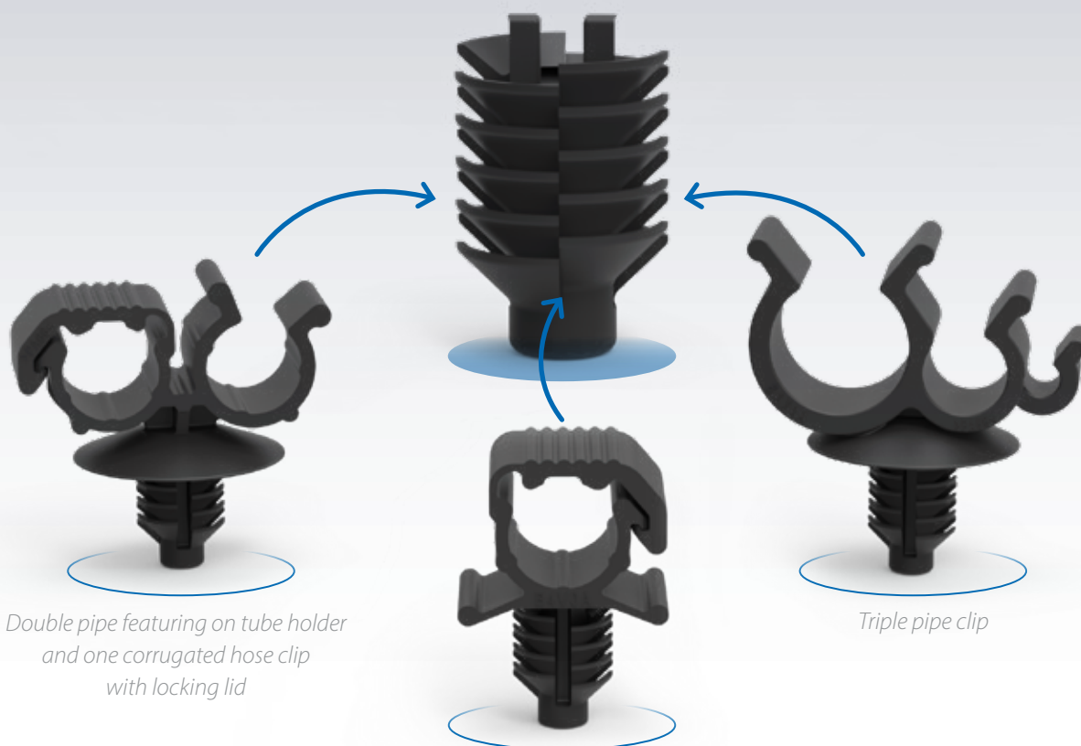
Pipe and hose clip with locking lid
